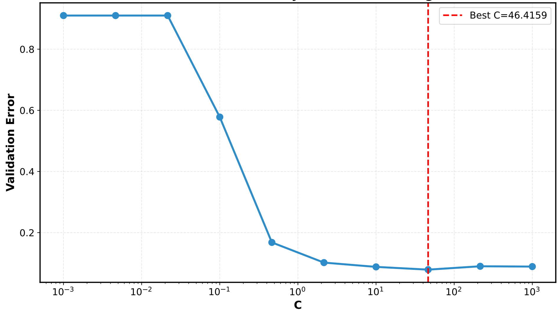
Validation Error vs C (Polynomial Kernel, degree=1)
